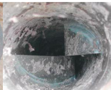
Statiflo NR Sludge mixer after 90 hours operation
